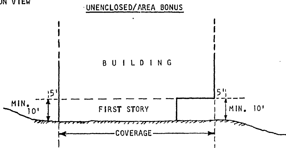
ILLUSTRATION "B" ELEVATION VIEW
