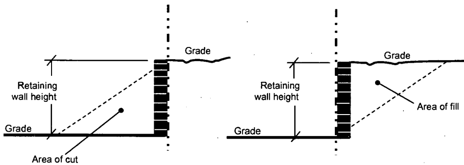
Diagram 113-02QQ Retaining Wall Height
