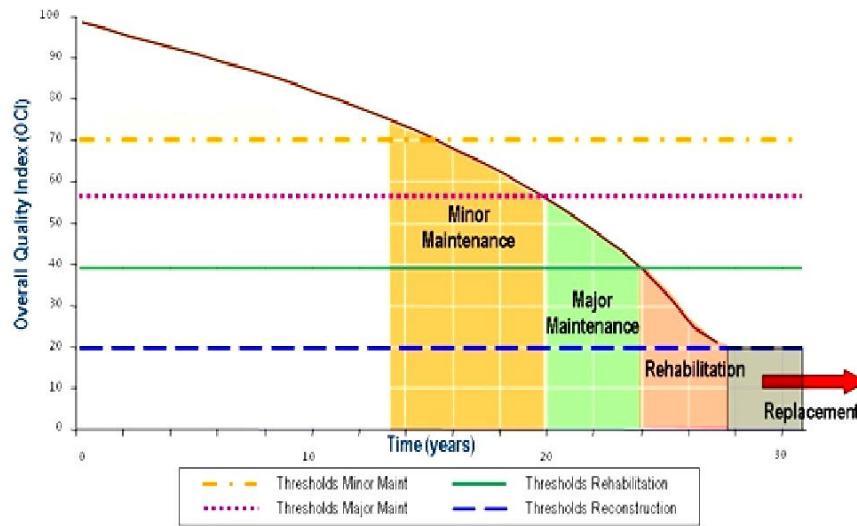
Chart 1: Pavement Lifecycle
